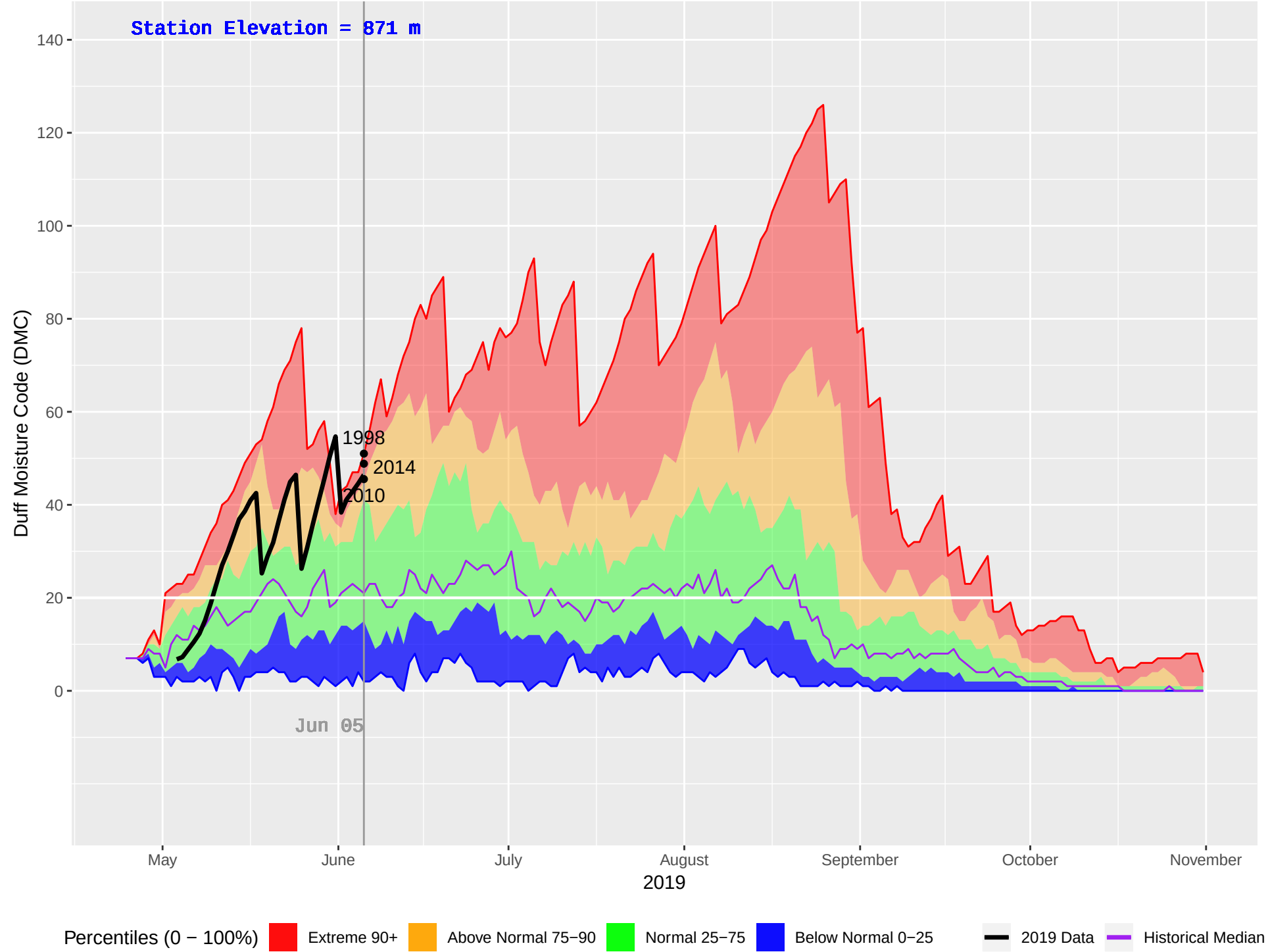
SUSTUT (156) : Historical (1989–2018), Current (2019) Daily Duff Moisture Code (DMC)
