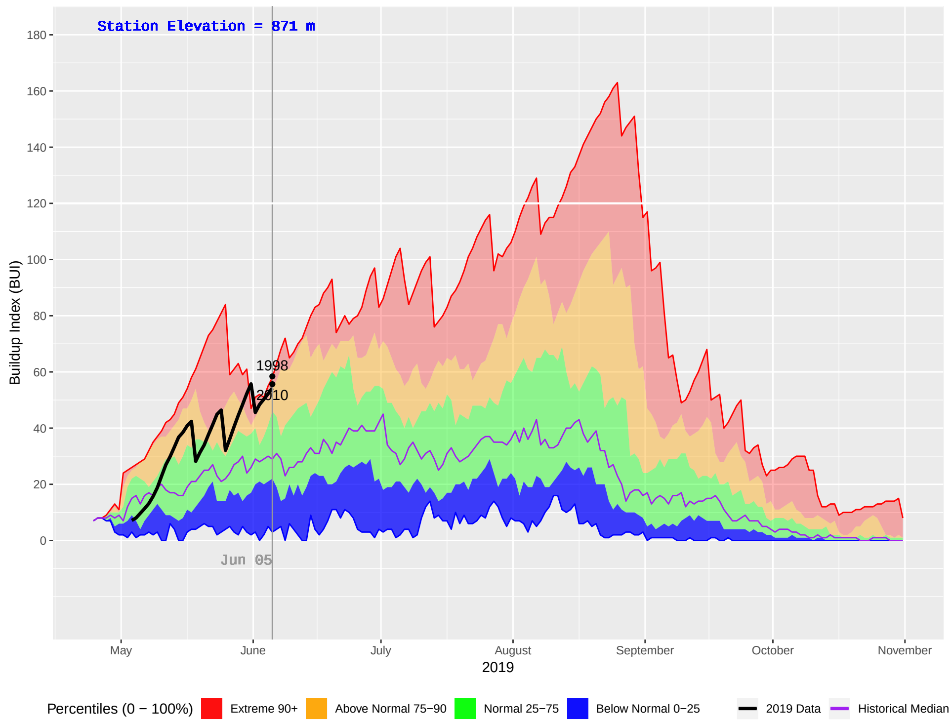
SUSTUT (156) : Historical (1989–2018), Current (2019) Daily Buildup Index (BUI)
