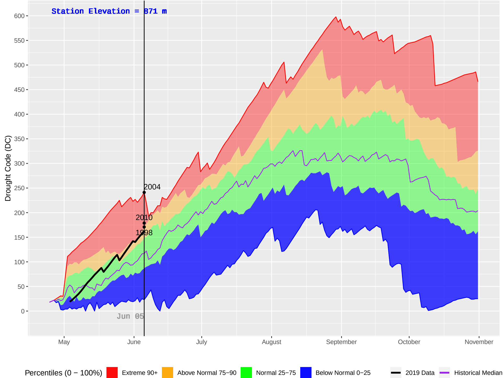
SUSTUT (156) : Historical (1989–2018) and Current (2019) Daily Drought Code (DC)
