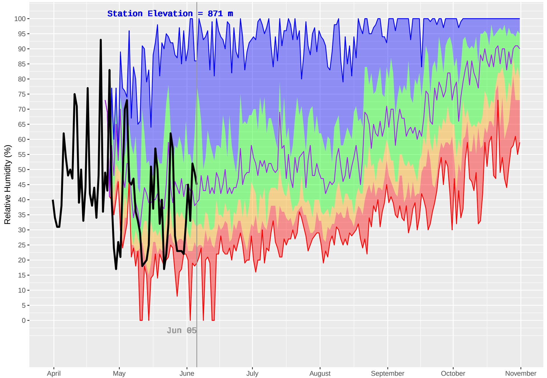
SUSTUT (156) : Historical (1989–2018) and Current (2019) Daily Relative Humidity
